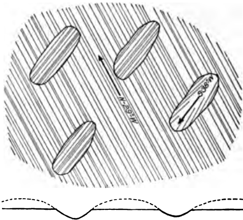
FIG. 330. — Limestone surface at Sibley, Michigan.
